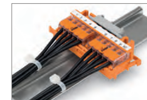
Vertical mounting with strain relief plate on DIN rail; wiring locations identified by marker strips
